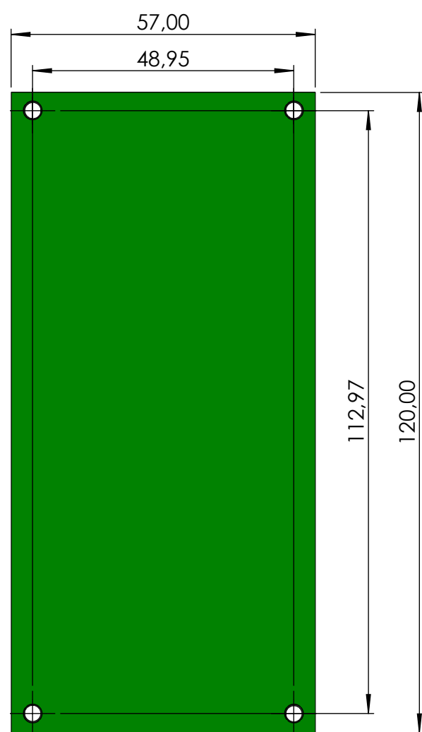
PCB MAX SIZE
