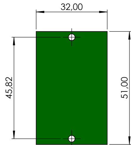
PCB MAX SIZE
